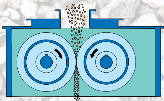
Sectional drawing of Double Roll Crusher fitted with smooth rolls
