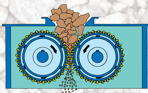
Sectional drawing of Double Roll Crusher fitted with toothed rolls
